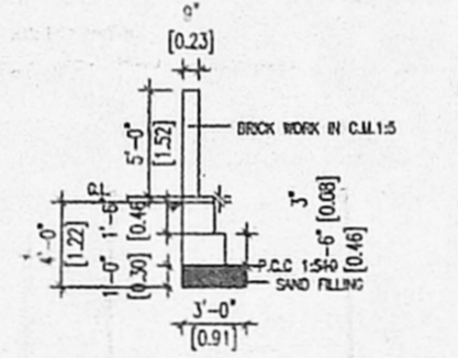
CROSS SEC. OF COMPOUND WALL
