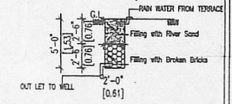
RAIN WATER HARVEST
