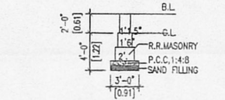
R.R.MASONRY DETAILS
